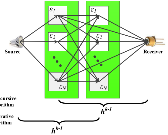
Fig. 5. Recursive and Iterative models.
